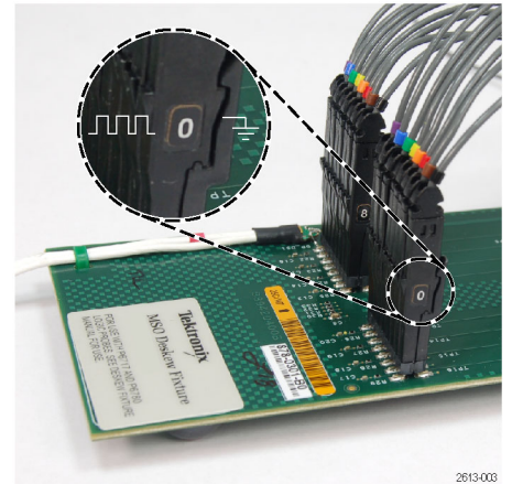
Figure 3: Single-ended probe connections
