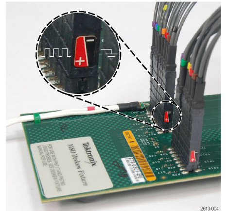
Figure 4: Differential probe connections
